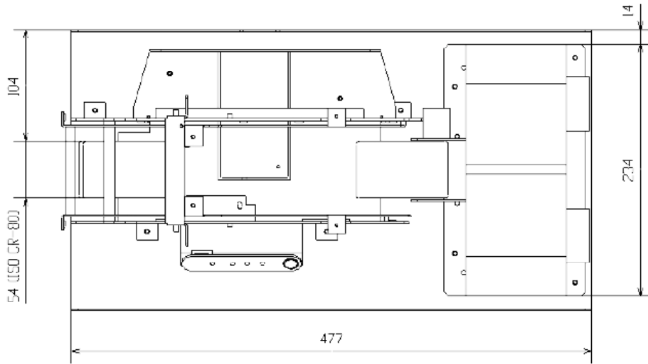
Printer Module Seen from above
