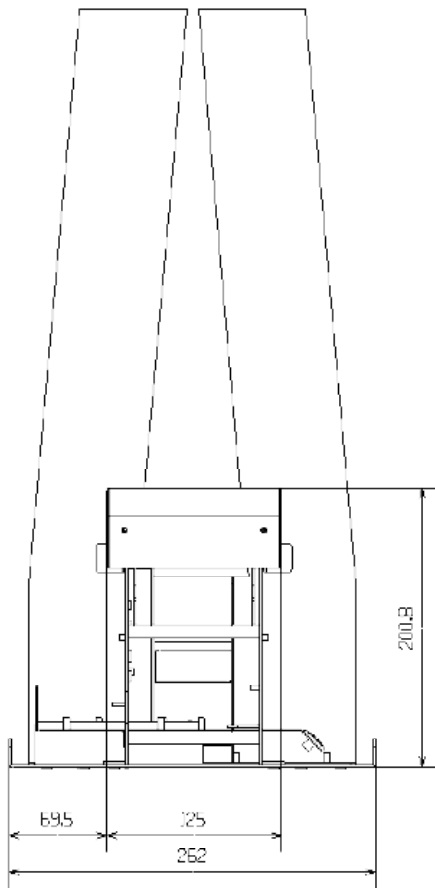
Card Feeder Module Seen from back
