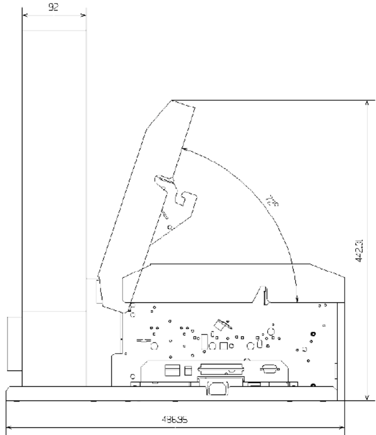
Printer Module Opening Angle
